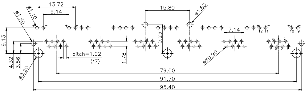
PC Board Layout(t=1.60) Component Side Shown
